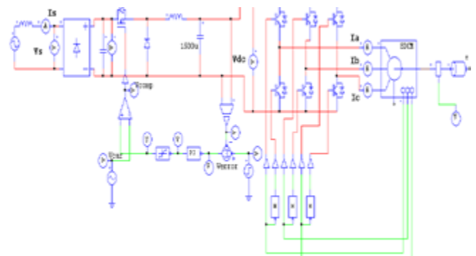
FIGURE 9: PSIM Simulation of BLDC Motor Drive with Buck converters.
