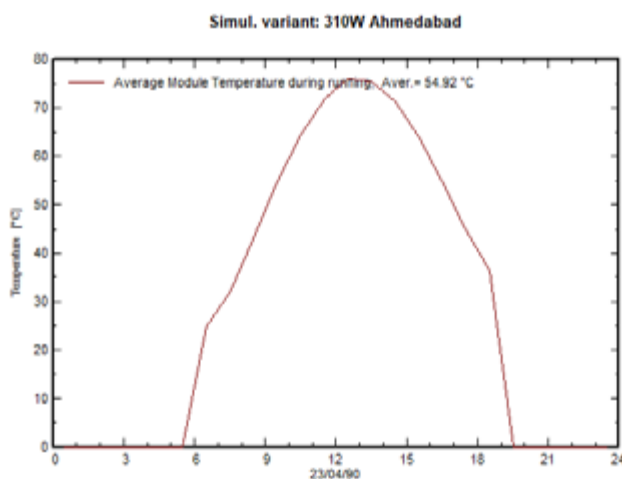
Figure 4: Solar PV module temperature rise in a summer day at Ahmedabad using PVSyst 6.88 (PVsyst, 2020)
