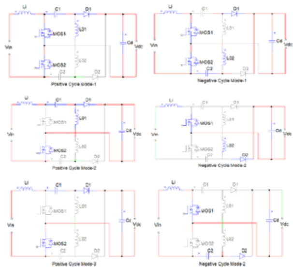
Fig-17 Operation of bridgeless SEPIC for different modes in a positive half cycle(a-b-c) and Negative half cycle(d-e-f)
